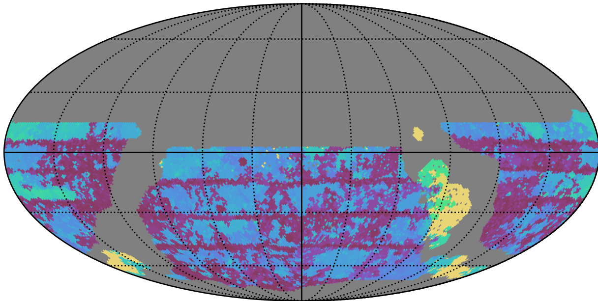
ddf_loaded_half_fl2_v3.4_10yrs WFD u band: Max Inter-Night Gap
