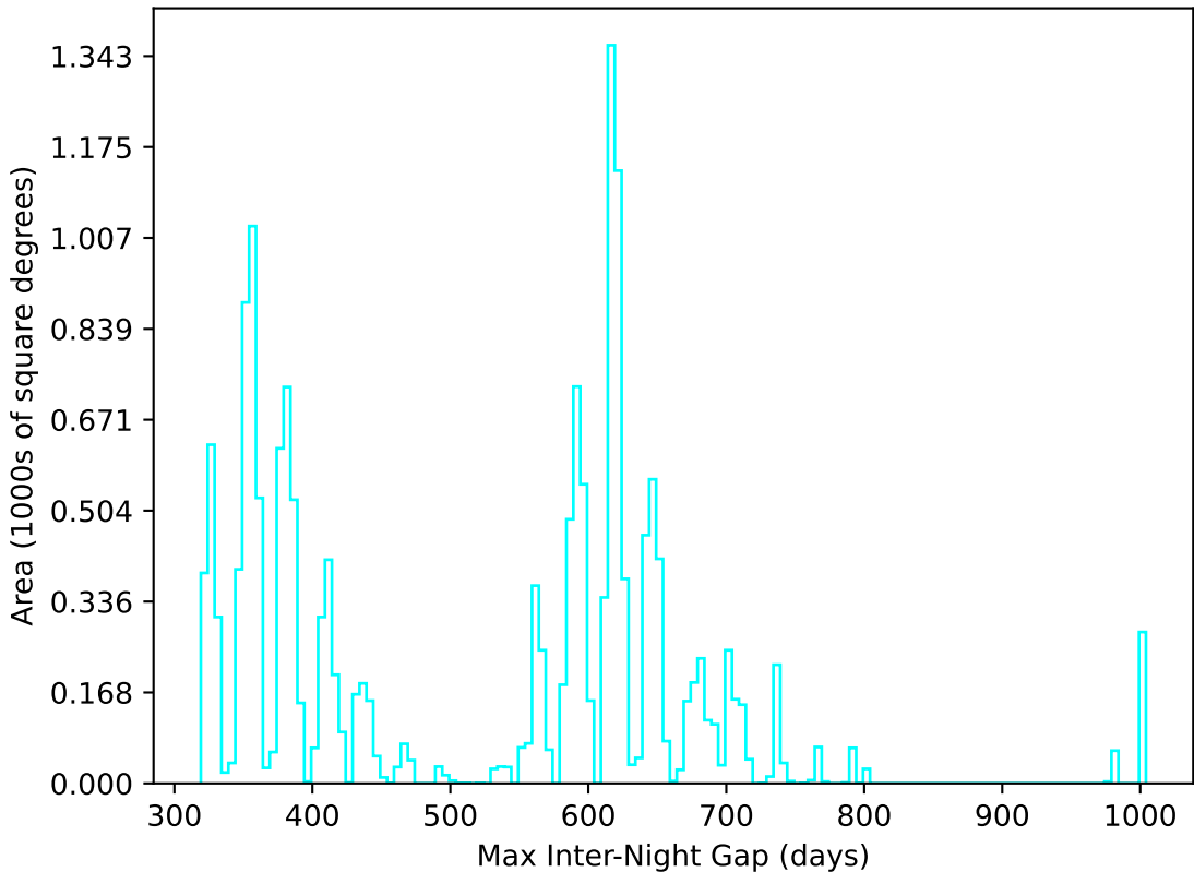
ddf_loaded_half_fl2_v3.4_10yrs WFD u band: Max Inter-Night Gap
