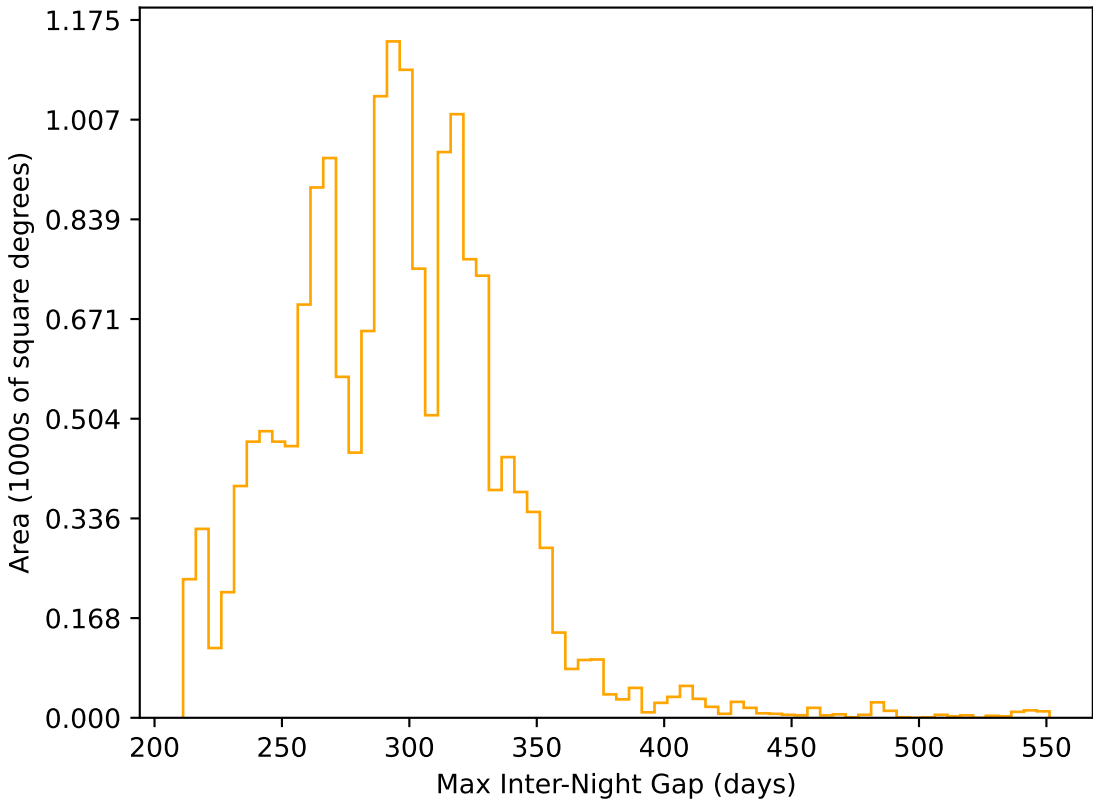
ddf_loaded_half_fl2_v3.4_10yrs WFD r band: Max Inter-Night Gap
