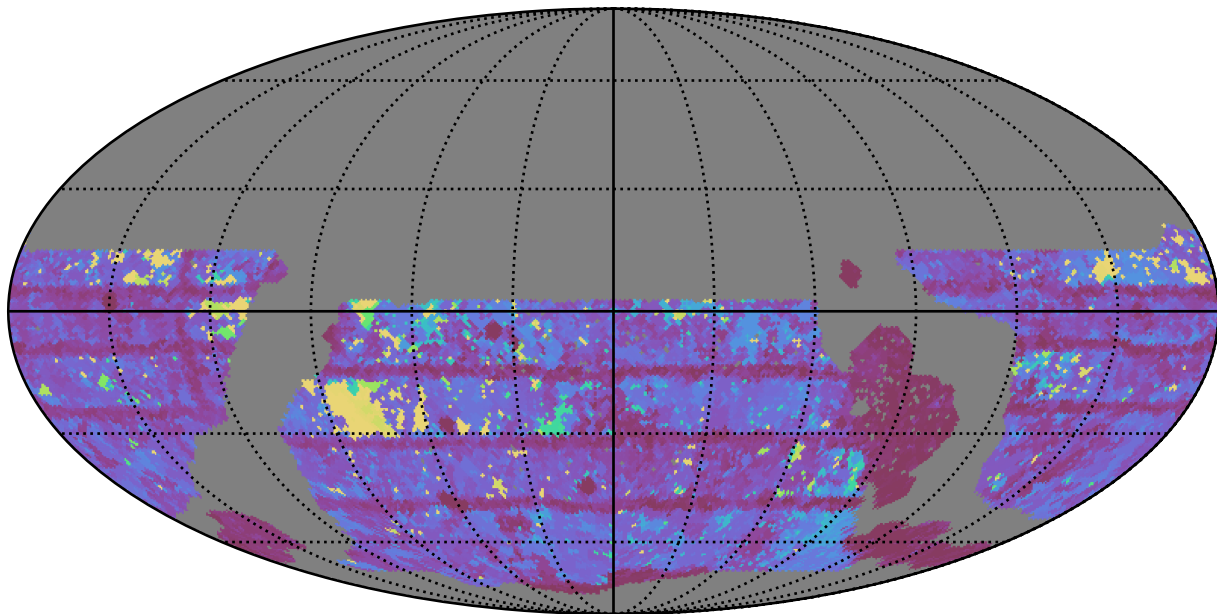
ddf_loaded_half_fl2_v3.4_10yrs WFD i band: Max Inter-Night Gap
