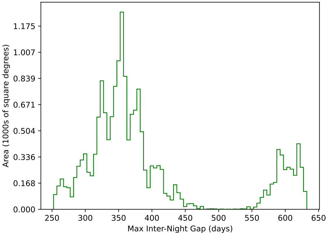
ddf_loaded_half_fl2_v3.4_10yrs WFD g band: Max Inter-Night Gap
