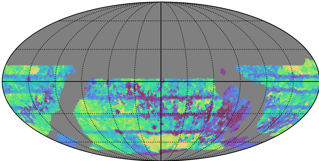
ddf_loaded_half_fl2_v3.4_10yrs WFD all bands: Max Inter-Night Gap
