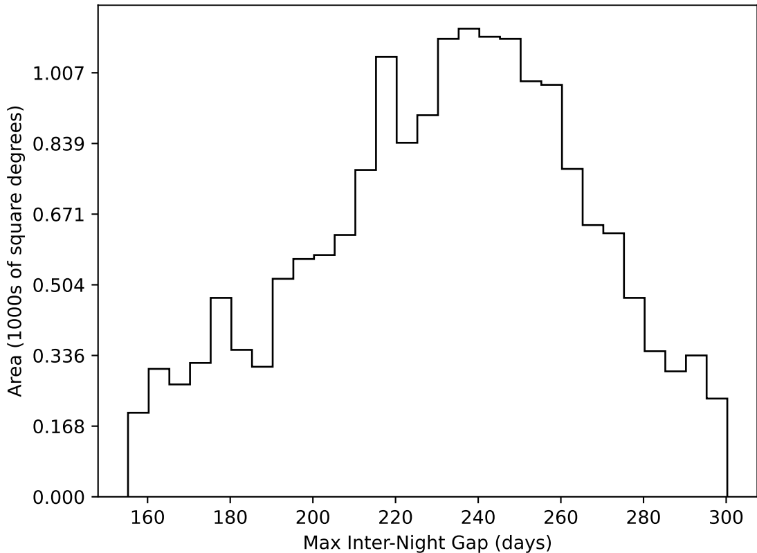
ddf_loaded_half_fl2_v3.4_10yrs WFD all bands: Max Inter-Night Gap
