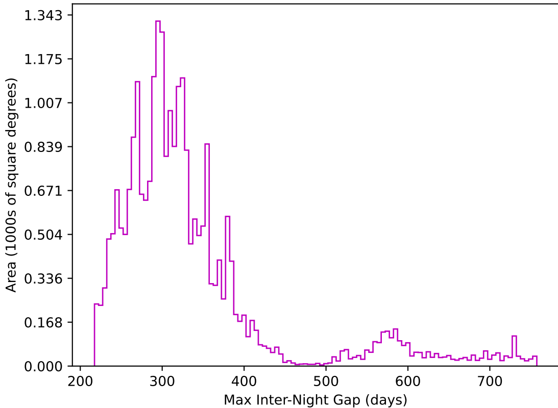
ddf_loaded_half_fl2_v3.4_10yrs All sky z band: Max Inter-Night Gap
