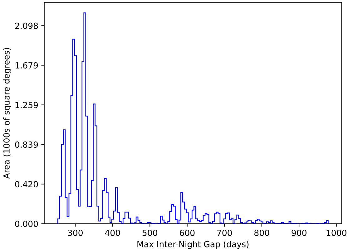
ddf_loaded_half_fl2_v3.4_10yrs All sky y band: Max Inter-Night Gap
