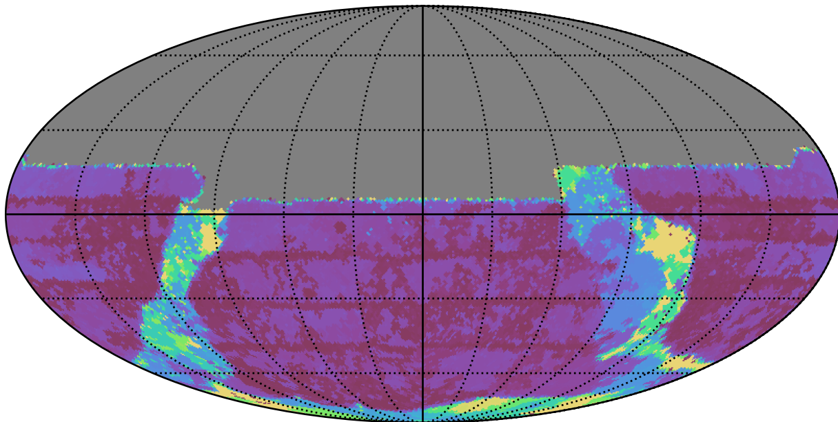
ddf_loaded_half_fl2_v3.4_10yrs All sky u band: Max Inter-Night Gap
