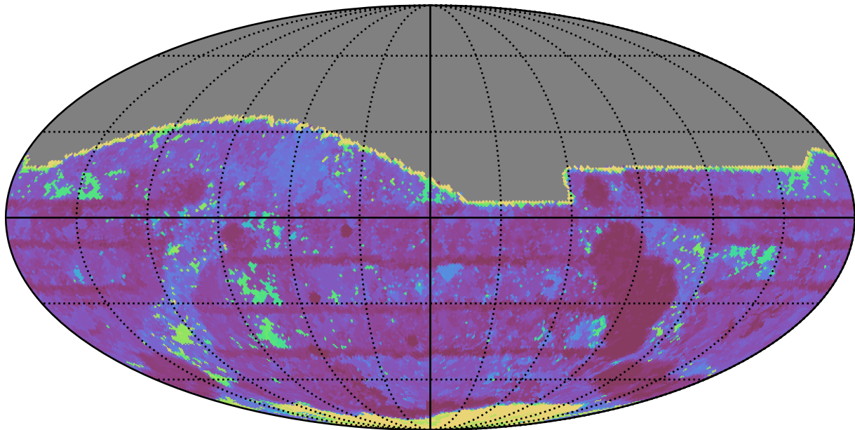
ddf_loaded_half_fl2_v3.4_10yrs All sky r band: Max Inter-Night Gap
