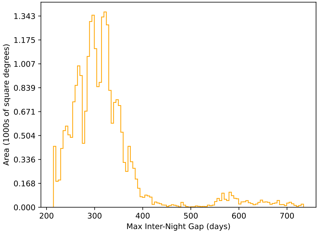
ddf_loaded_half_fl2_v3.4_10yrs All sky r band: Max Inter-Night Gap
