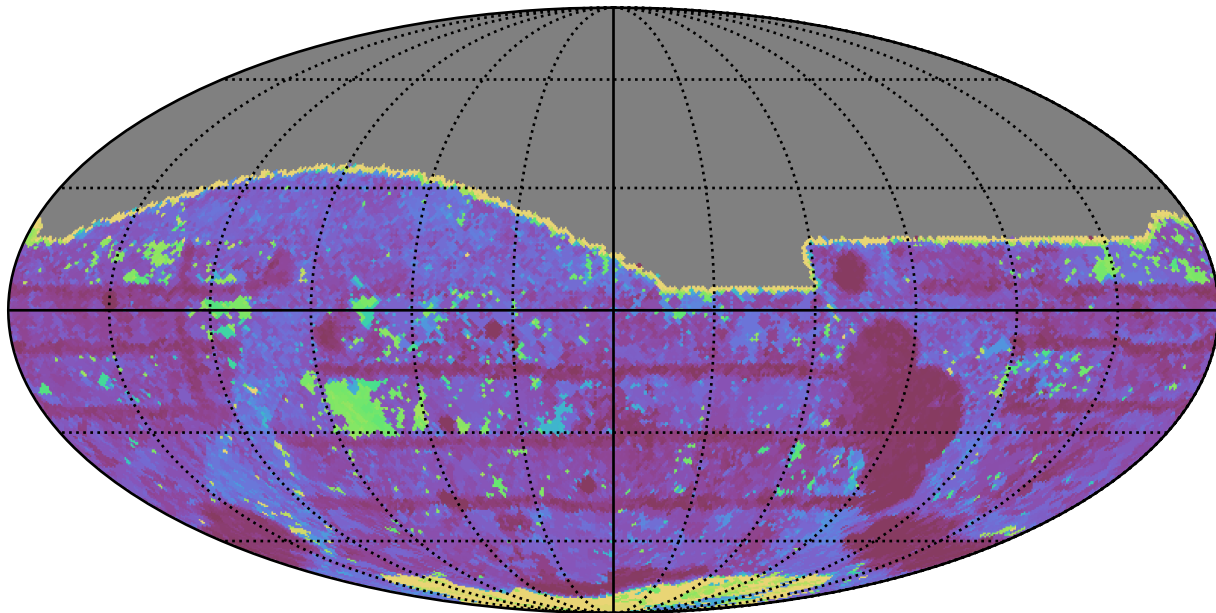
ddf_loaded_half_fl2_v3.4_10yrs All sky i band: Max Inter-Night Gap
