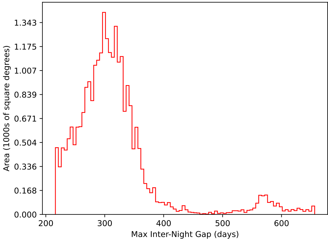
ddf_loaded_half_fl2_v3.4_10yrs All sky i band: Max Inter-Night Gap
