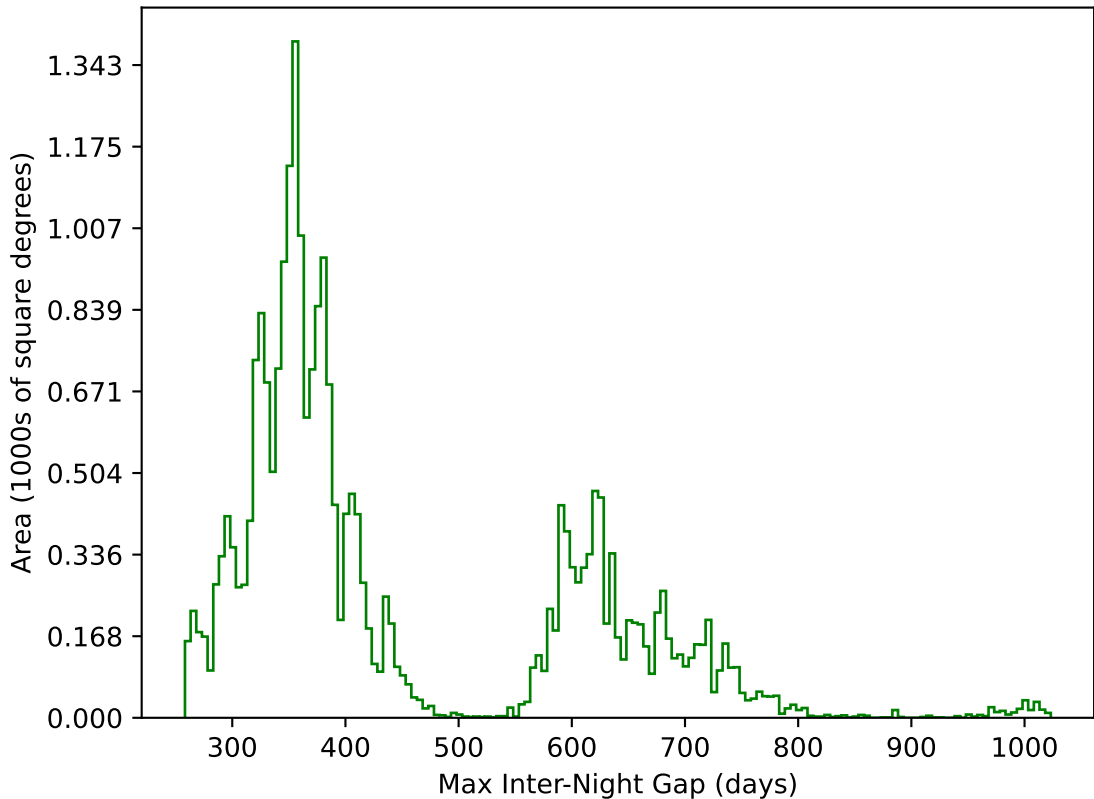
ddf_loaded_half_fl2_v3.4_10yrs All sky g band: Max Inter-Night Gap
