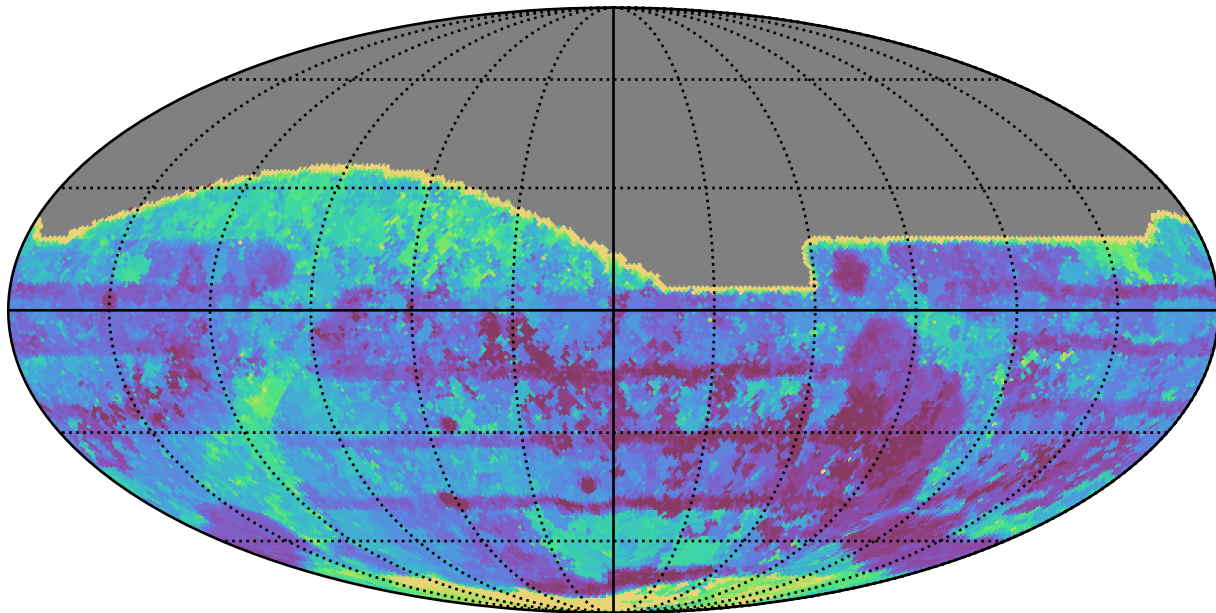
ddf_loaded_half_fl2_v3.4_10yrs All sky all bands: Max Inter-Night Gap
