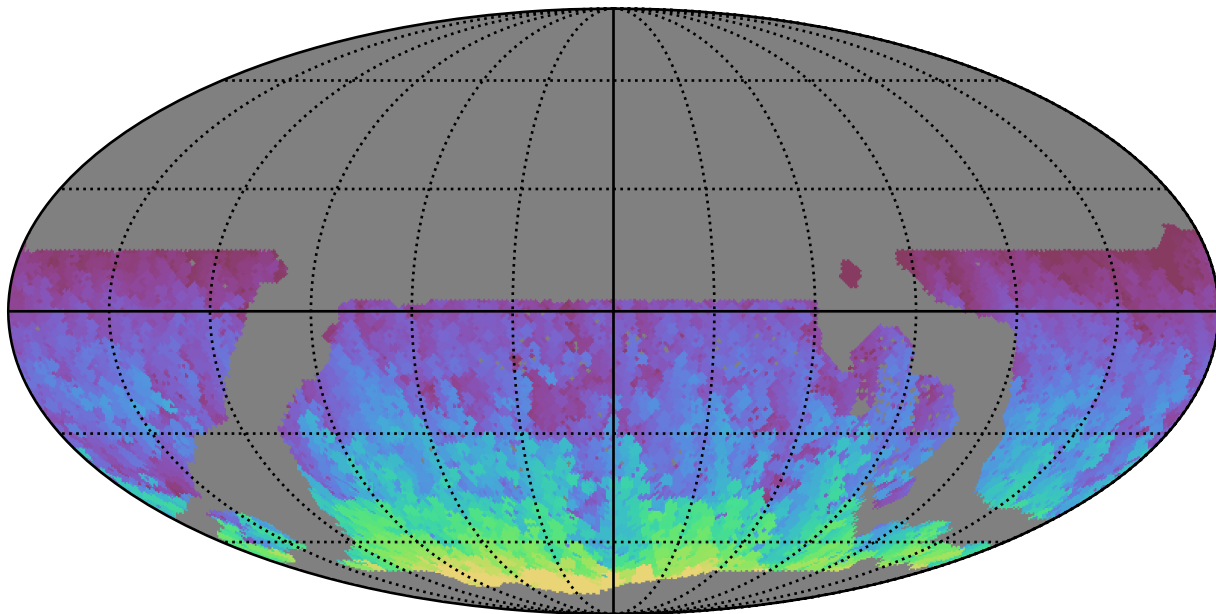
ddf_loaded_half_fl2_v3.4_10yrs WFD y band: Max HA
