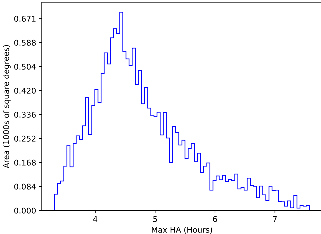
ddf_loaded_half_fl2_v3.4_10yrs WFD y band: Max HA
