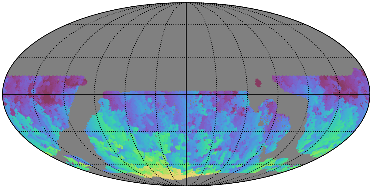
ddf_loaded_half_fl2_v3.4_10yrs WFD u band: Max HA
