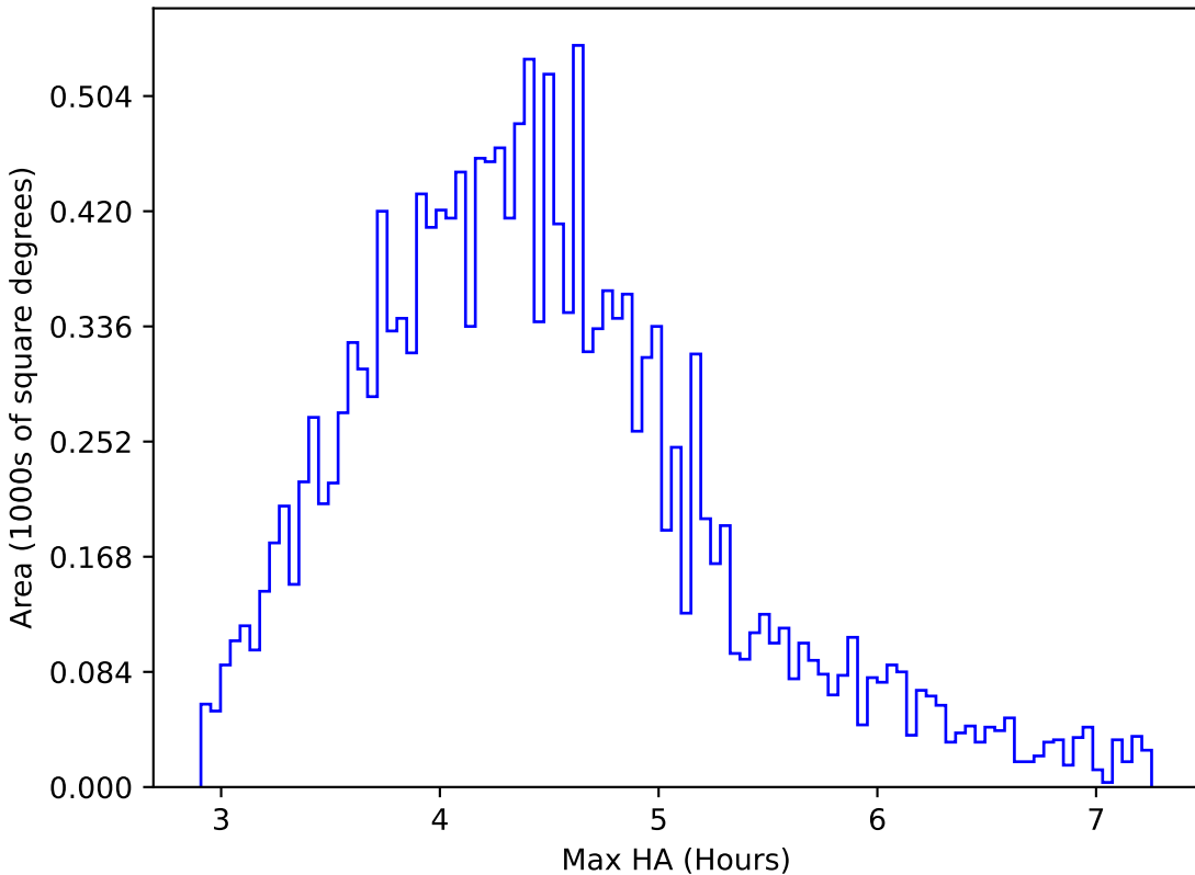
ddf_loaded_half_fl2_v3.4_10yrs WFD r band: Max HA
