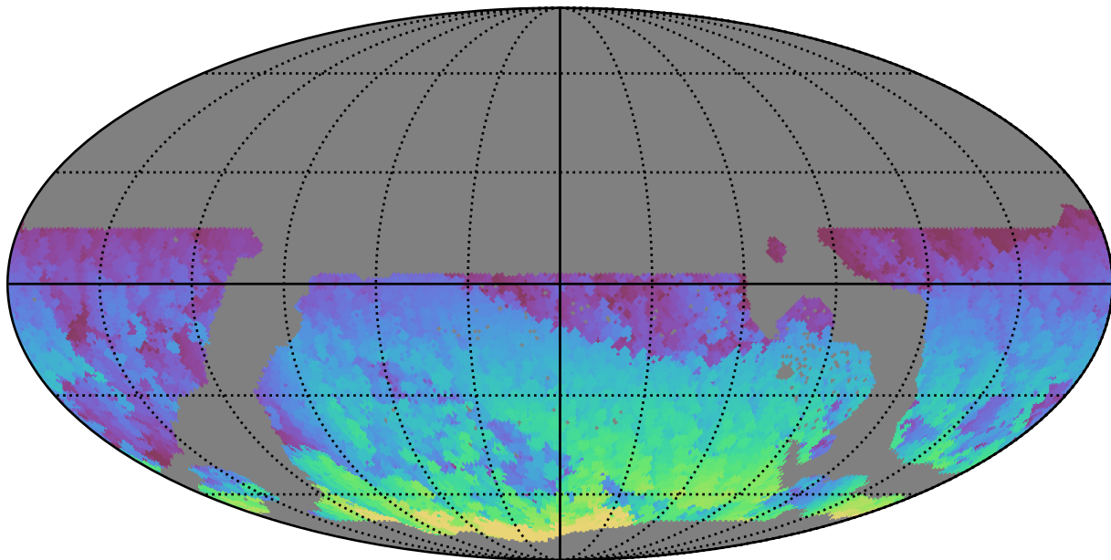
ddf_loaded_half_fl2_v3.4_10yrs WFD i band: Max HA
