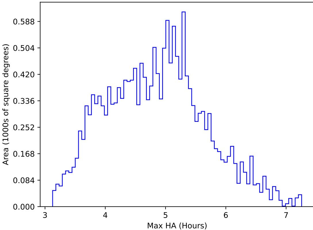
ddf_loaded_half_fl2_v3.4_10yrs WFD i band: Max HA
