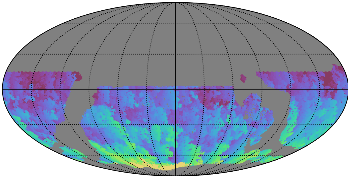
ddf_loaded_half_fl2_v3.4_10yrs WFD g band: Max HA
