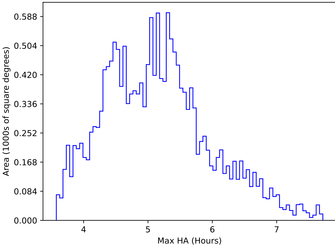
ddf_loaded_half_fl2_v3.4_10yrs WFD all bands: Max HA
