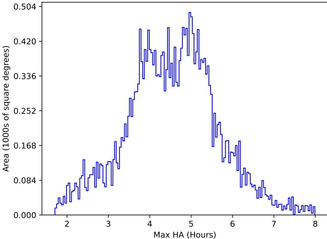
ddf_loaded_half_fl2_v3.4_10yrs All sky z band: Max HA
