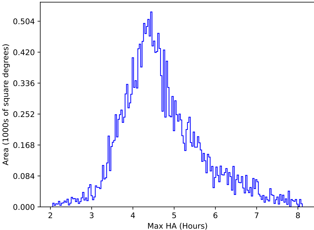
ddf_loaded_half_fl2_v3.4_10yrs All sky y band: Max HA
