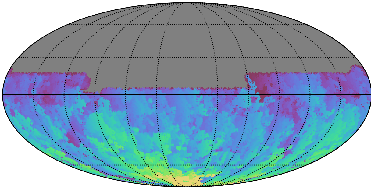
ddf_loaded_half_fl2_v3.4_10yrs All sky u band: Max HA
