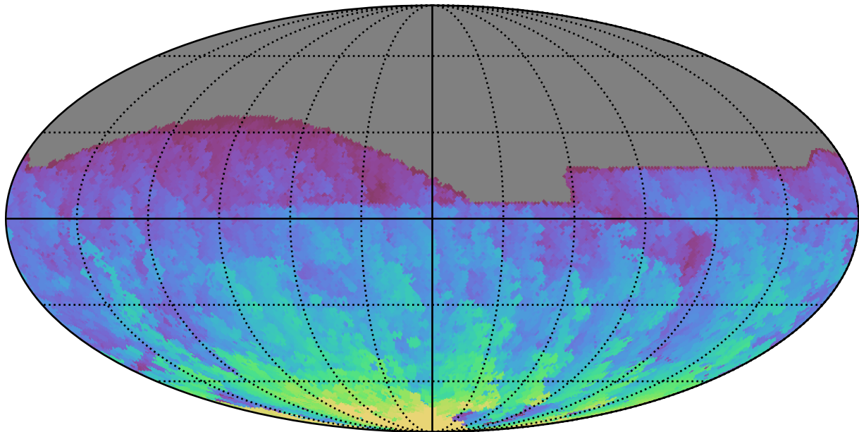
ddf_loaded_half_fi2_v3.4_10yrs All sky r band: Max HA
