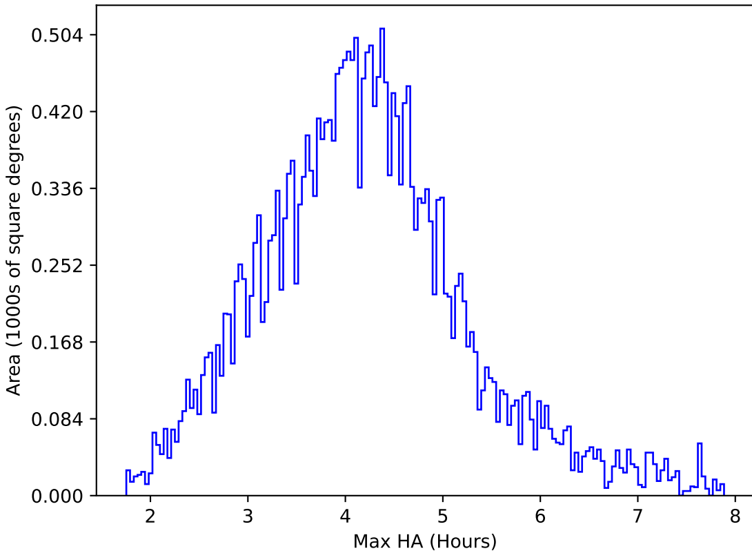
ddf_loaded_half_fl2_v3.4_10yrs All sky r band: Max HA
