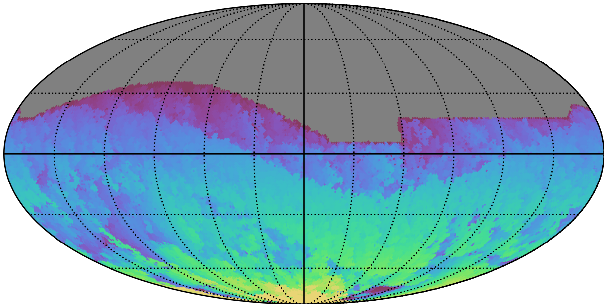
ddf_loaded_half_f12_v3.4_10yrs All sky i band: Max HA
