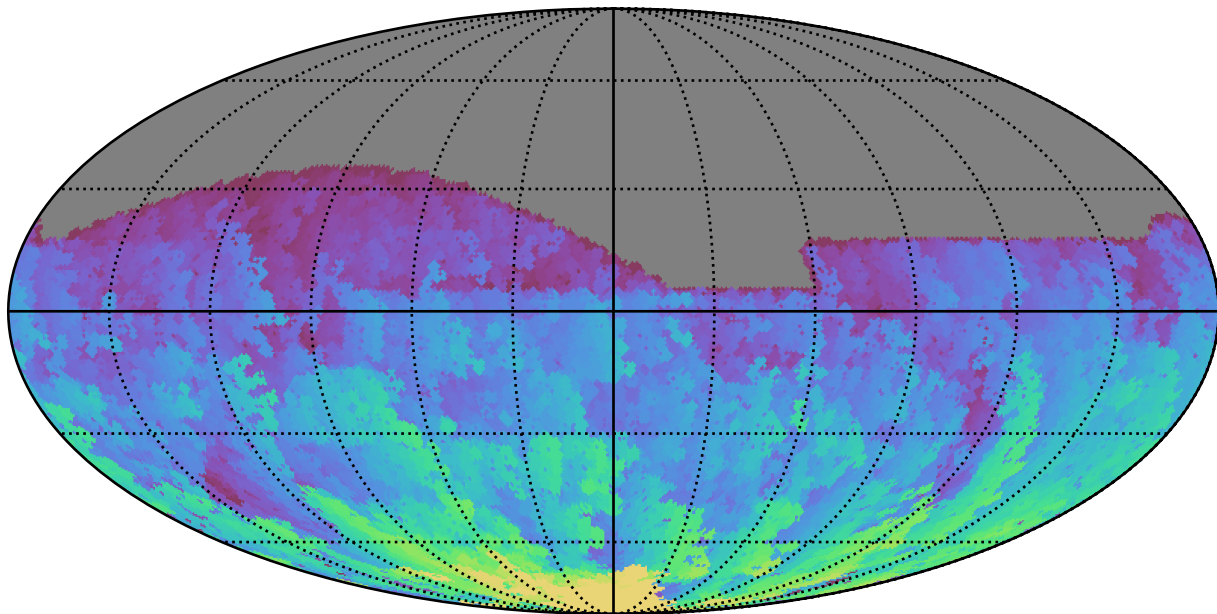
ddf_loaded_half_fl2_v3.4_10yrs All sky g band: Max HA
