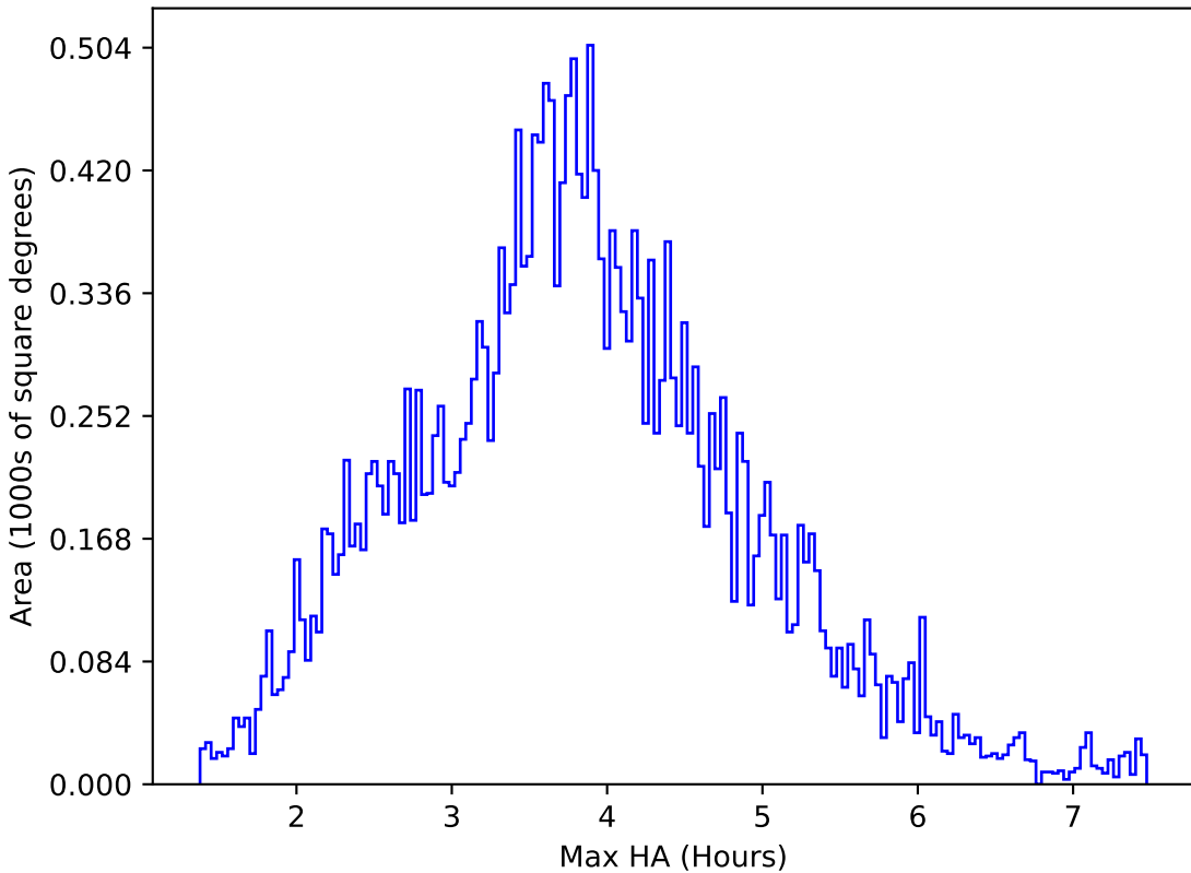
ddf_loaded_half_fl2_v3.4_10yrs All sky g band: Max HA
