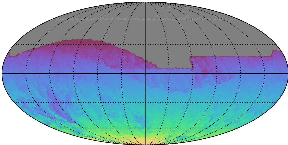
ddf_loaded_half_fl2_v3.4_10yrs All sky all bands: Max HA
