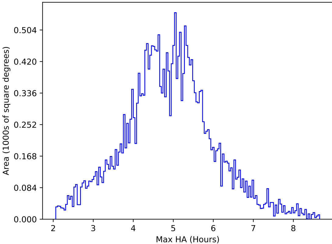
ddf_loaded_half_fl2_v3.4_10yrs All sky all bands: Max HA
