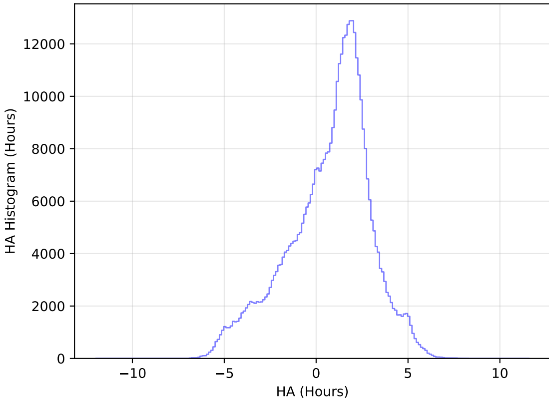
ddf_loaded_half_fl2_v3.4_10yrs WFD z band: HA Histogram
