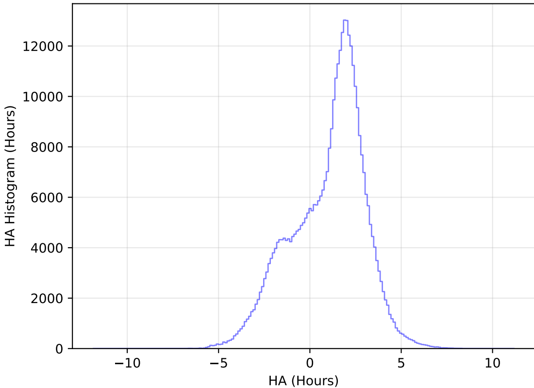
ddf_loaded_half_fl2_v3.4_10yrs WFD y band: HA Histogram
