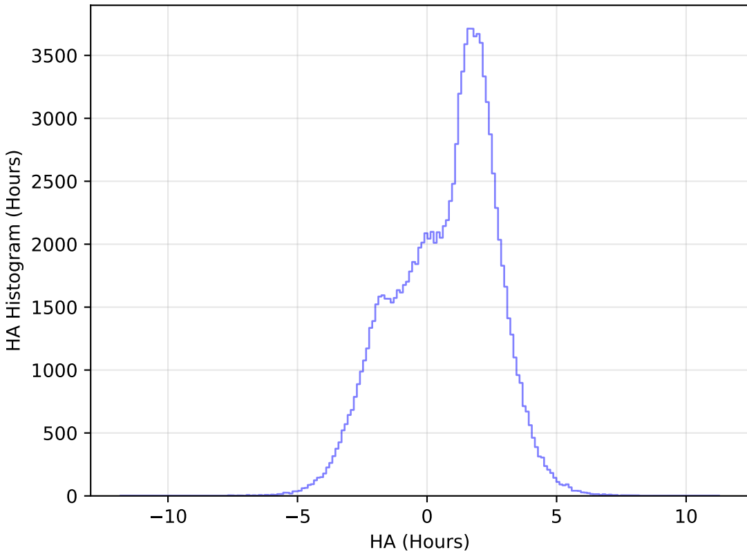
ddf_loaded_half_fl2_v3.4_10yrs WFD u band: HA Histogram
