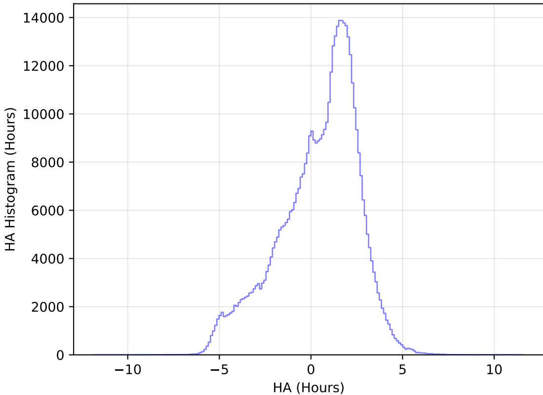
ddf_loaded_half_fl2_v3.4_10yrs WFD r band: HA Histogram
