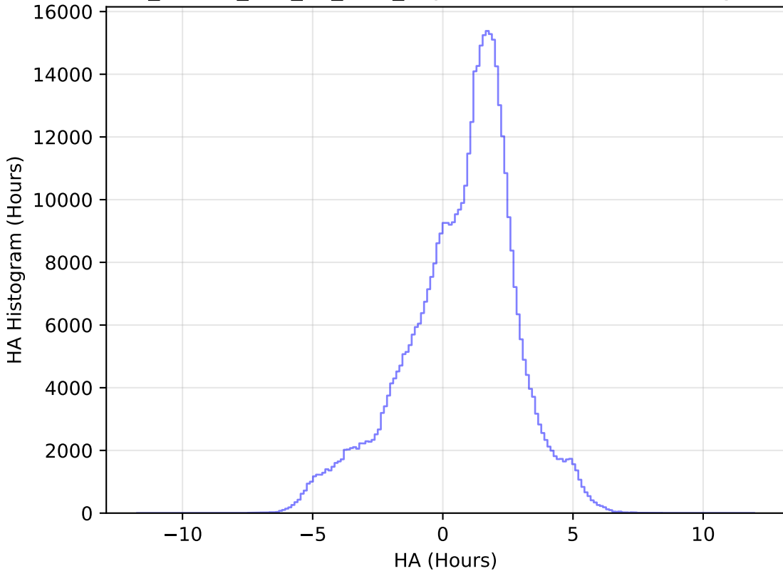
ddf_loaded_half_fl2_v3.4_10yrs WFD i band: HA Histogram
