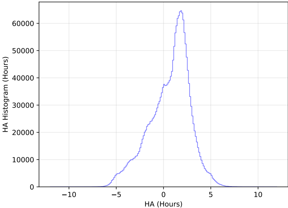
ddf_loaded_half_fl2_v3.4_10yrs WFD all bands: HA Histogram
