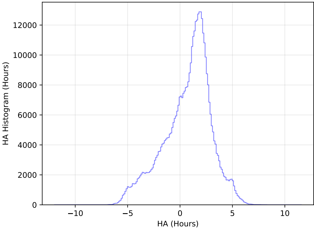
ddf_loaded_half_fl2_v3.4_10yrs All sky z band: HA Histogram
