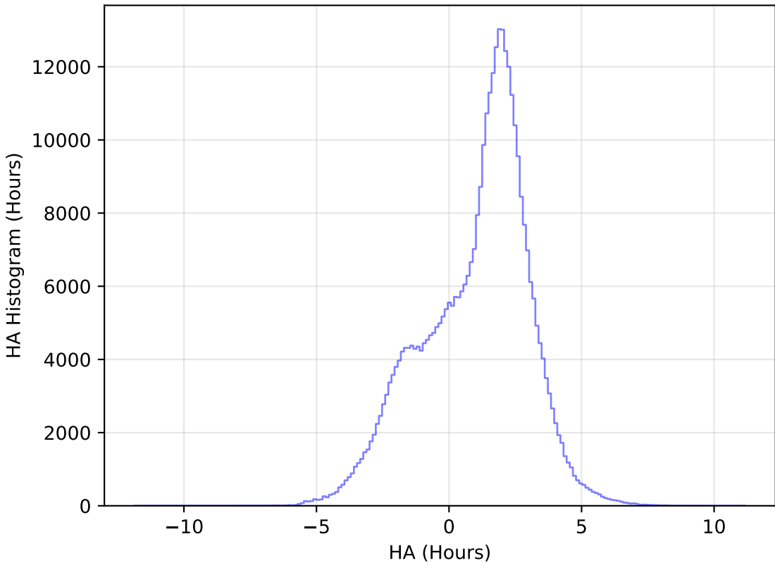
ddf_loaded_half_fl2_v3.4_10yrs All sky y band: HA Histogram
