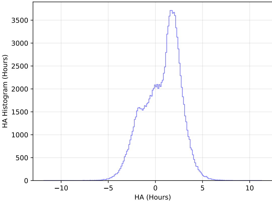
ddf_loaded_half_fl2_v3.4_10yrs All sky u band: HA Histogram
