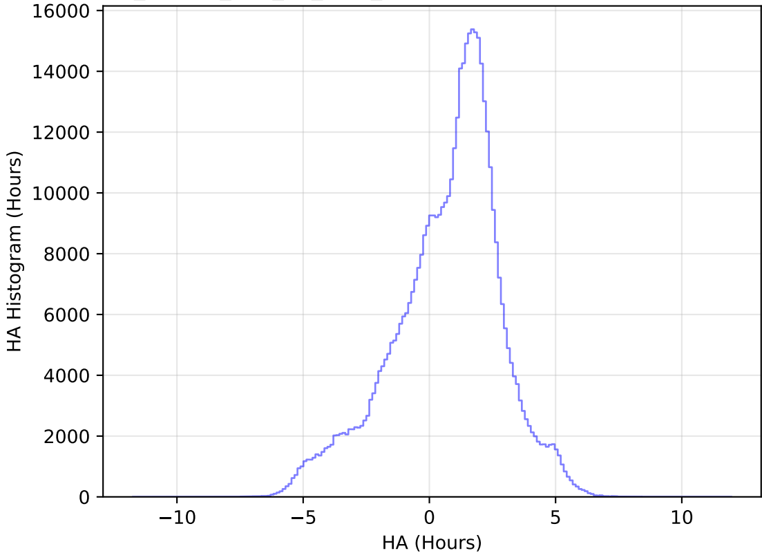
ddf_loaded_half_fl2_v3.4_10yrs All sky i band: HA Histogram
