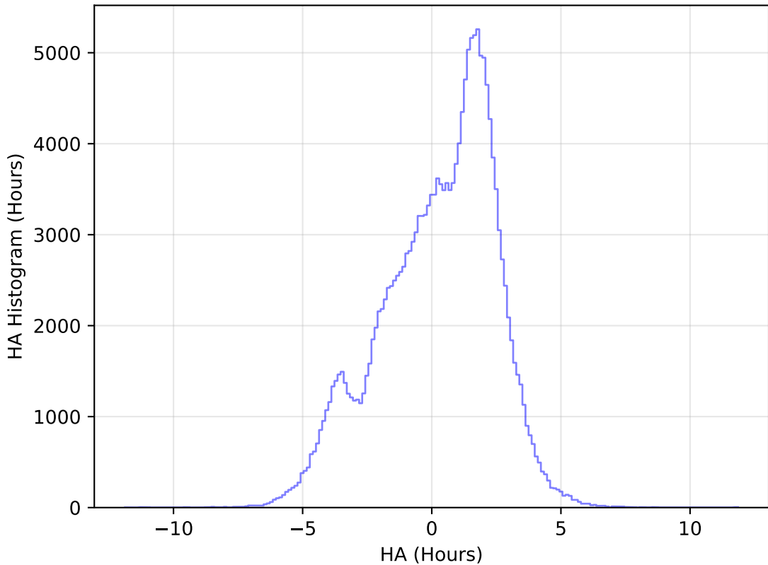
ddf_loaded_half_fl2_v3.4_10yrs All sky g band: HA Histogram
