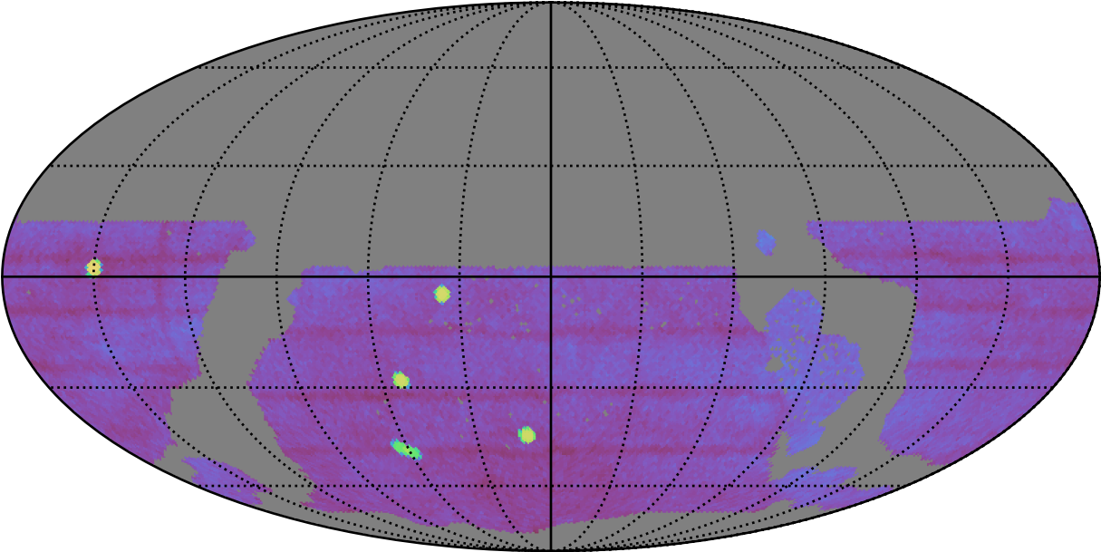
ddf_loaded_half_fl2_v3.4_10yrs gri WFD: Fraction of visits with a revisit < 60 min
