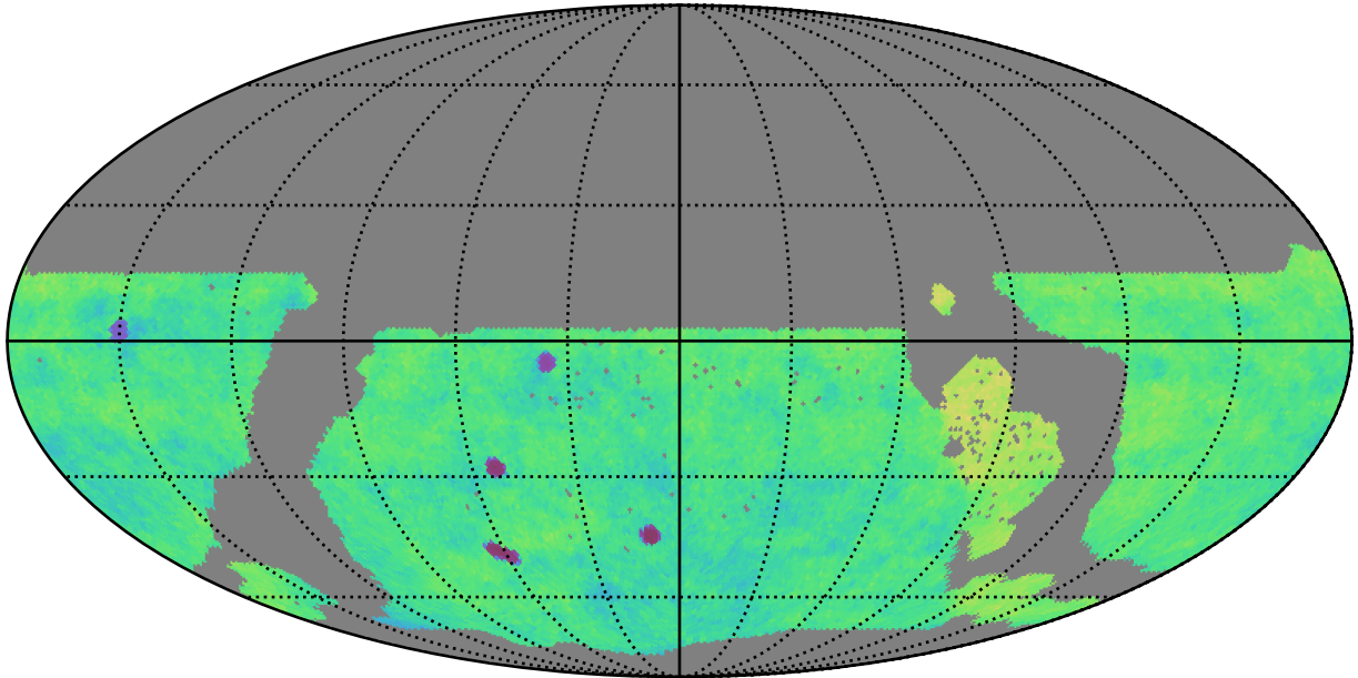
ddf_loaded_half_fl2_v3.4_10yrs gri WFD: Fraction of visits in pairs (10-60 min)
