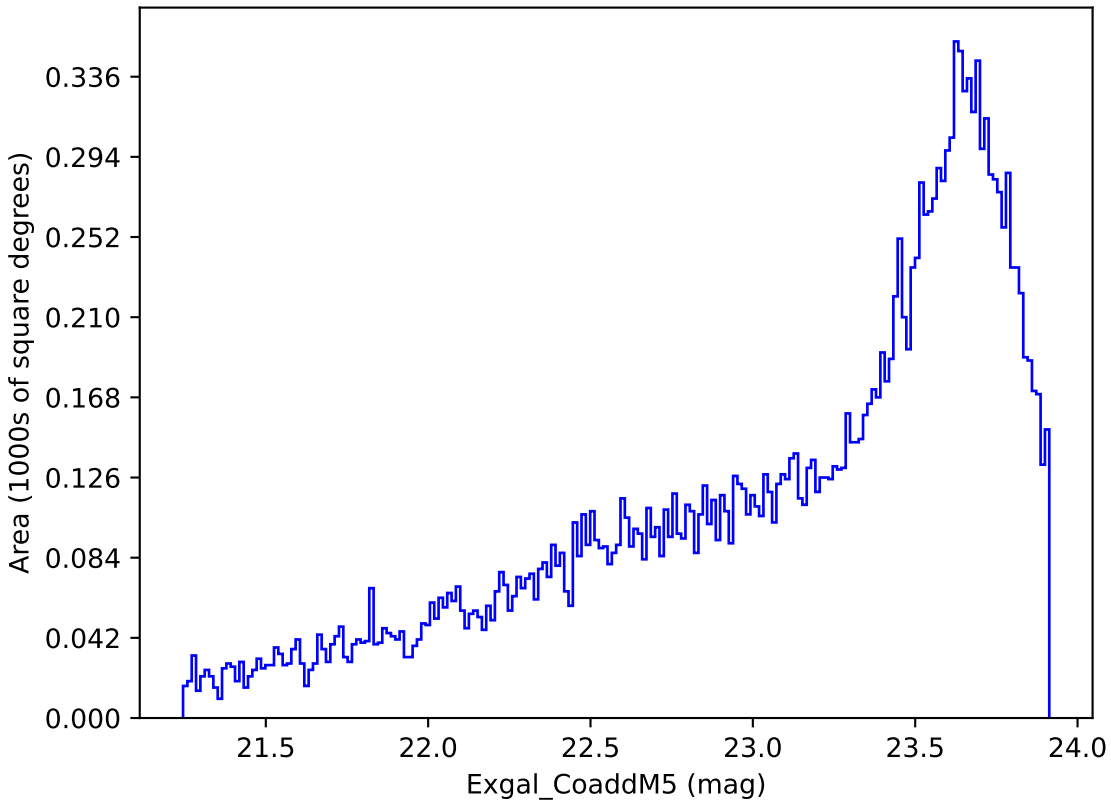
ddf_loaded_half_fl2_v3.4_10yrs Yr 3-4 y band: Exgal_CoaddM5
