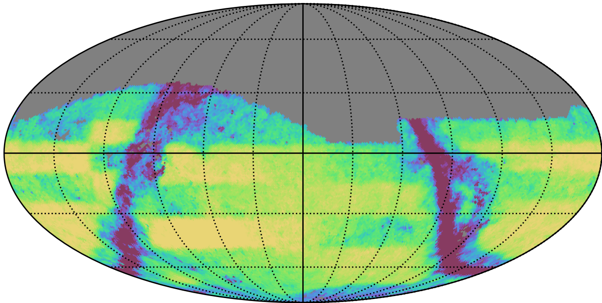
ddf_loaded_half_fl2_v3.4_10yrs Yr 3-4 r band: Exgal_CoaddM5
