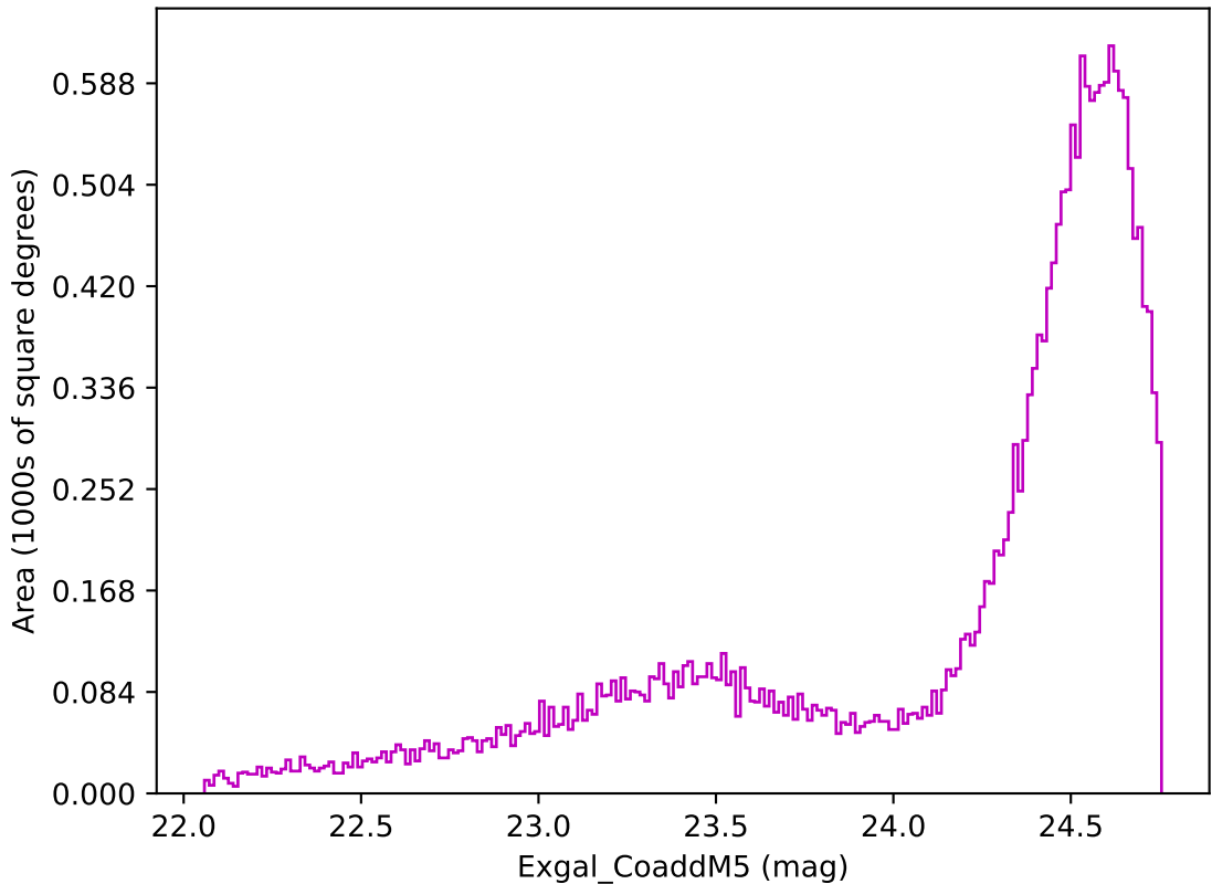
ddf_loaded_half_fl2_v3.4_10yrs Yr 1 z band: Exgal_CoaddM5
